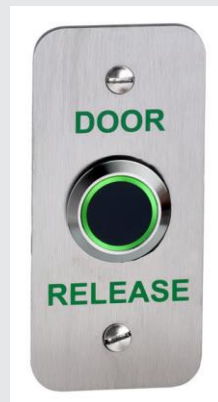
Flush mountable, narrow style, "TOUCH FREE" IP65 exit device, 12/24vdc, illuminated GREEN going RED, door open time 0.5 to 20 seconds, or toggle mode.
